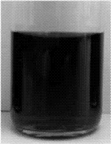
(B). Acetone
